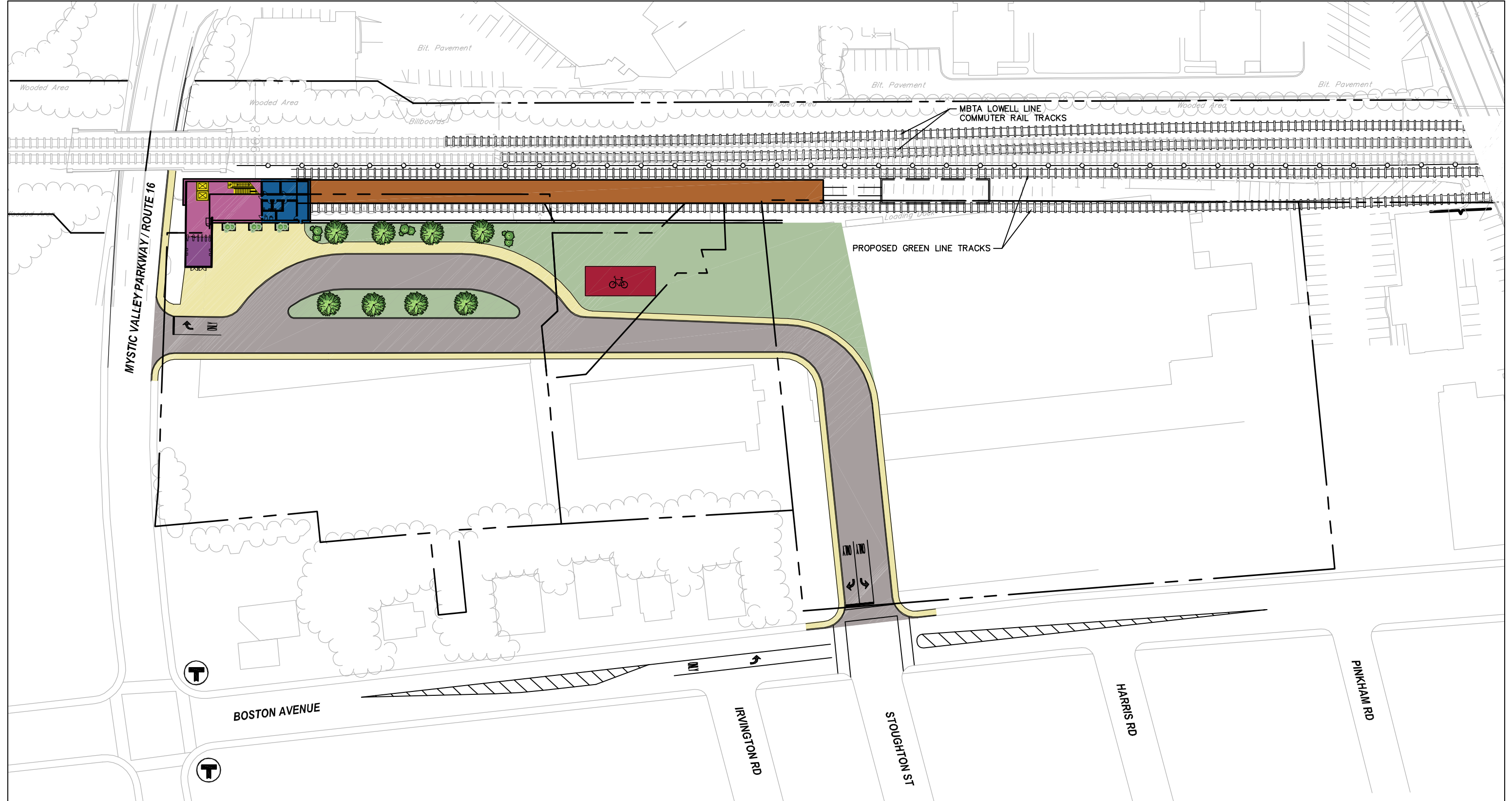
Figure 3.7-27 Mystic Valley Parkway / Route 16 Station Station Layout
