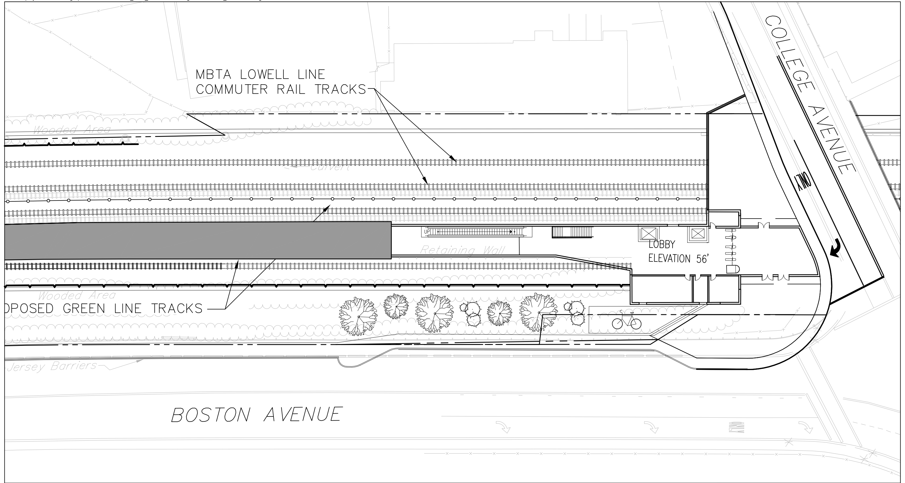
Figure 3.7-24 College Avenue Station Station Plan
