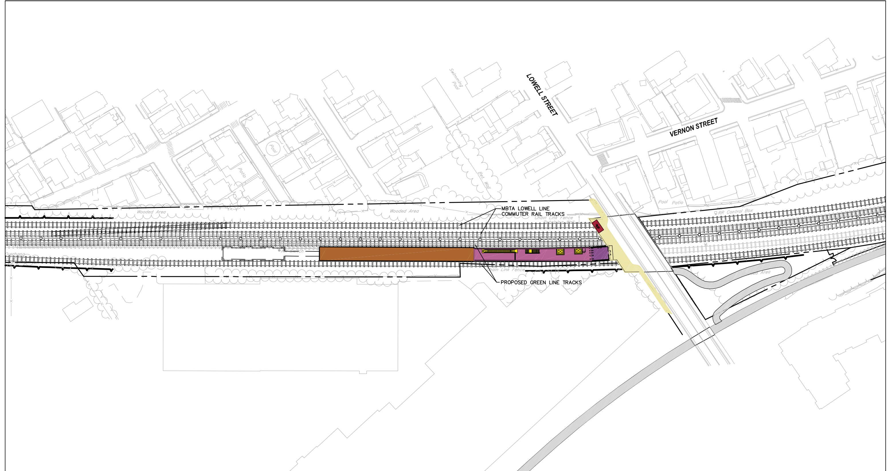
Figure 3.7-14 Lowell Street Station Station Layout
