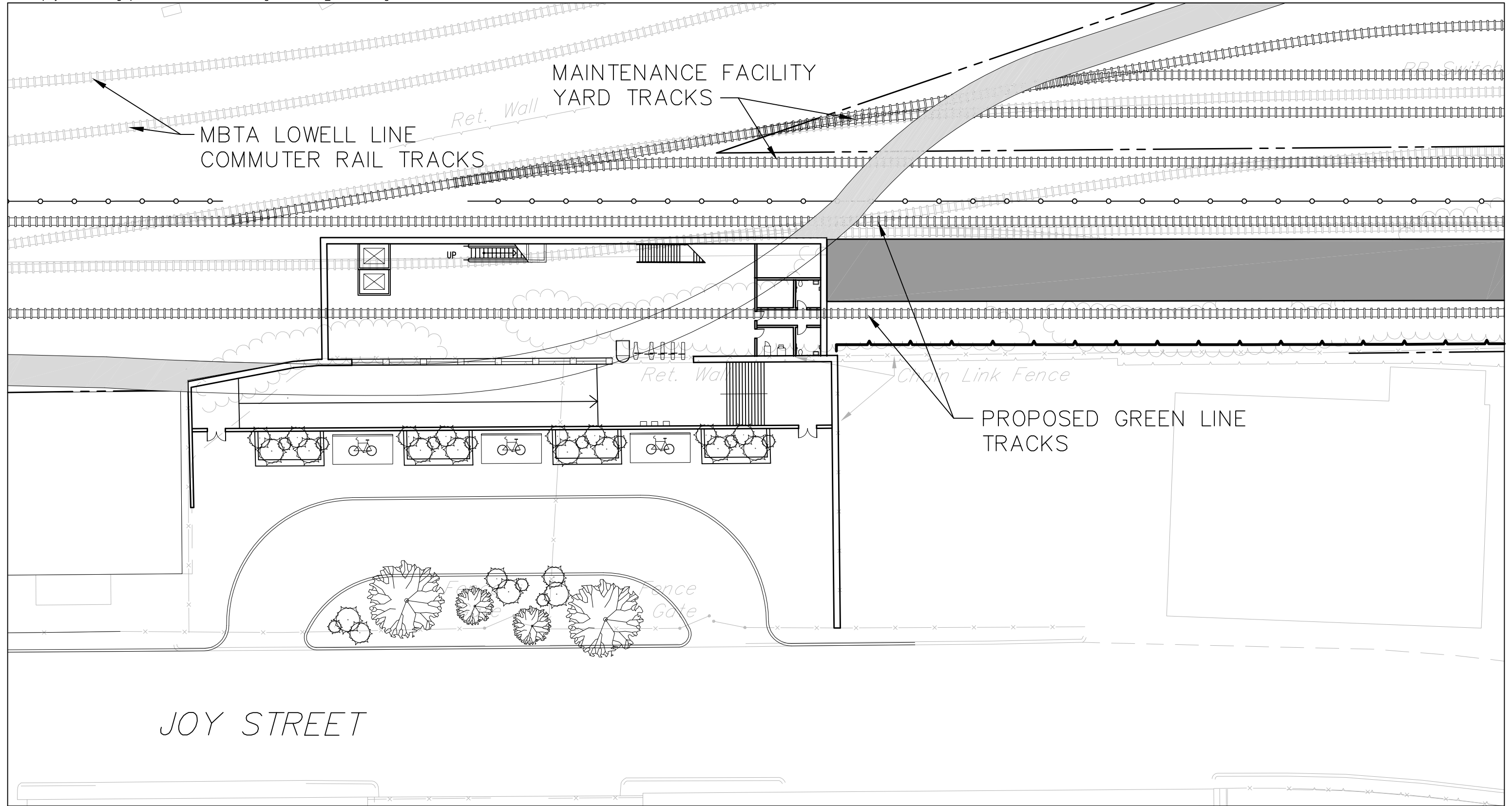
Figure 3.7-7 Brickbottom Station Station Plan
